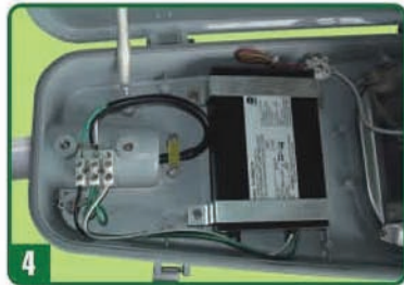
4 Fasten the cable with the cable press and connect the wire according to the wiring diagram.
